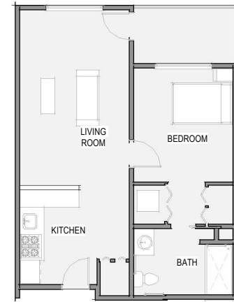
UNIT TYPE A1 1 BD/ 1 BA 725 sq. ft.
